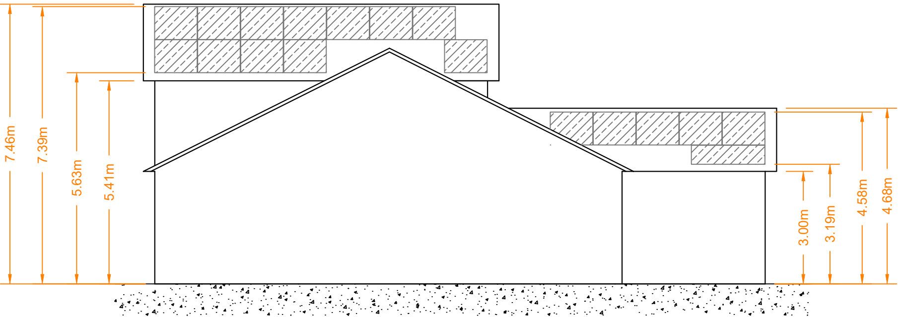
SOUTHWEST ELEVATION
